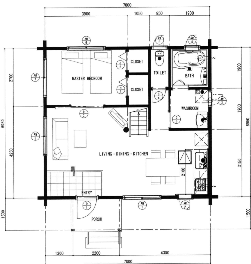
MAIN FLOOR
