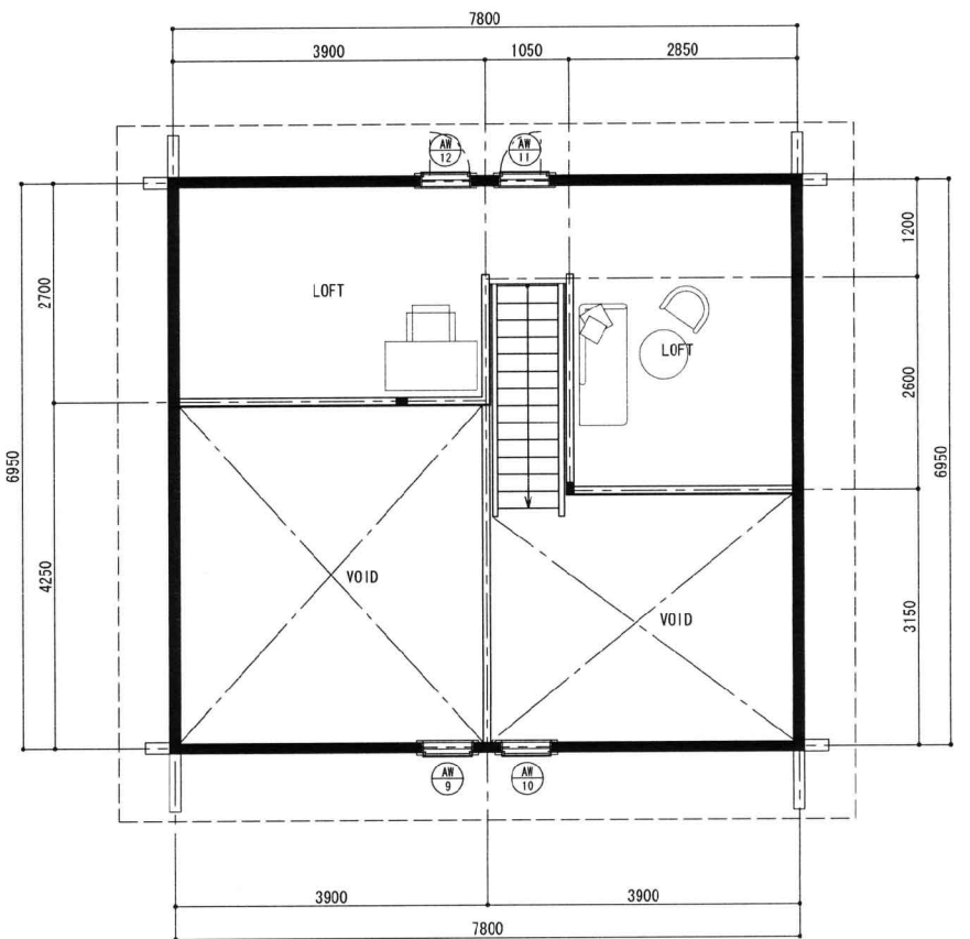
UPPER FLOOR
